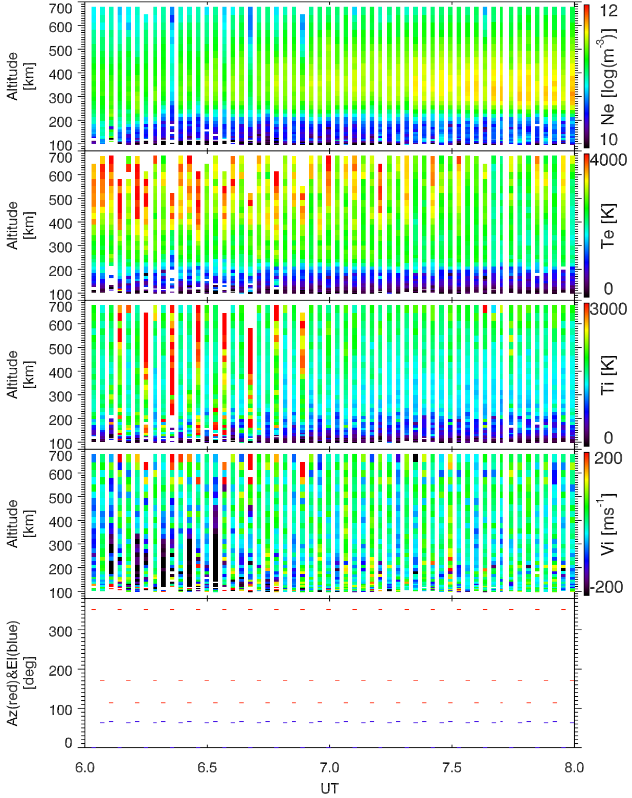
EISCAT 2002-10-18_06_08UT_tau0_ant@32m.
