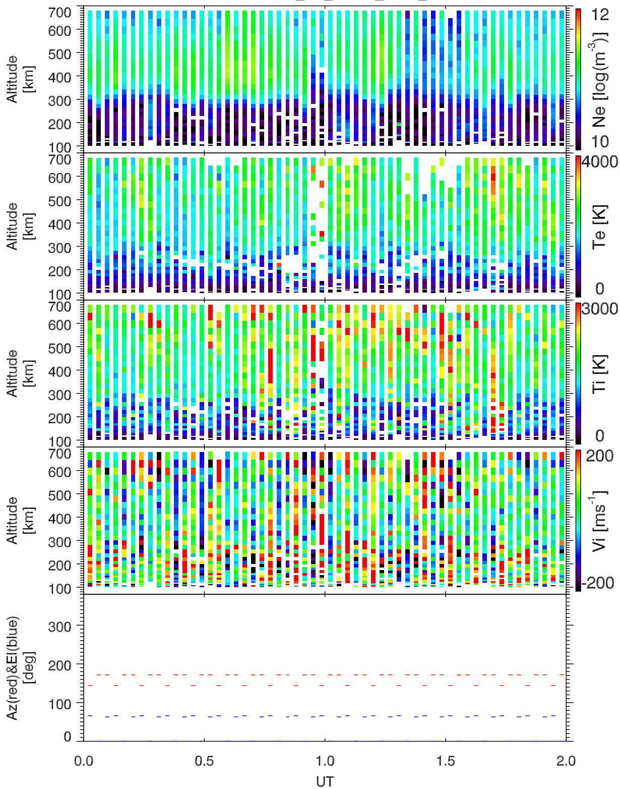
EISCAT 2002-10-19_00_02UT_tau0_ant@32m.
