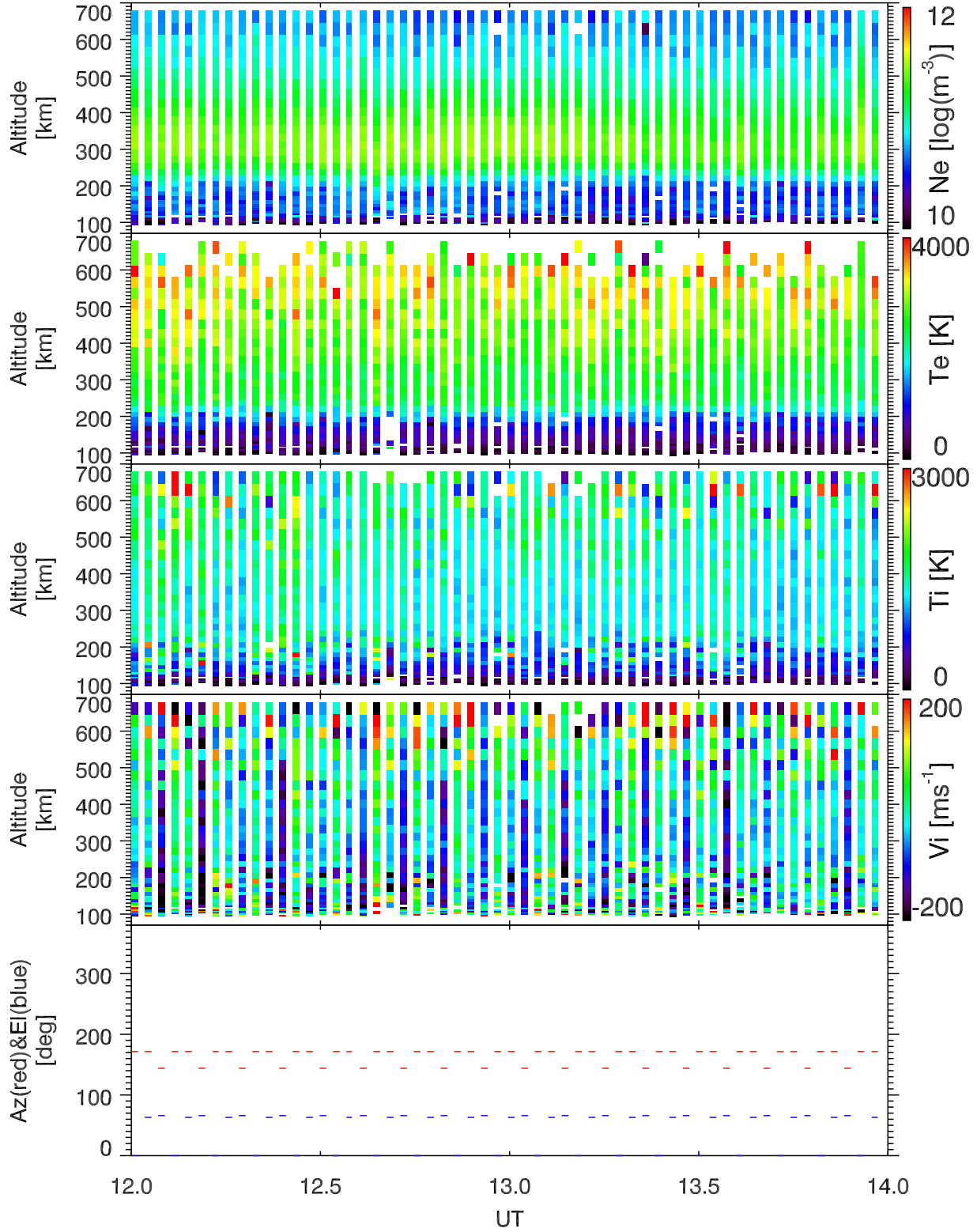
EISCAT 2002-10-19_12_14UT_tau0_ant@32m.
