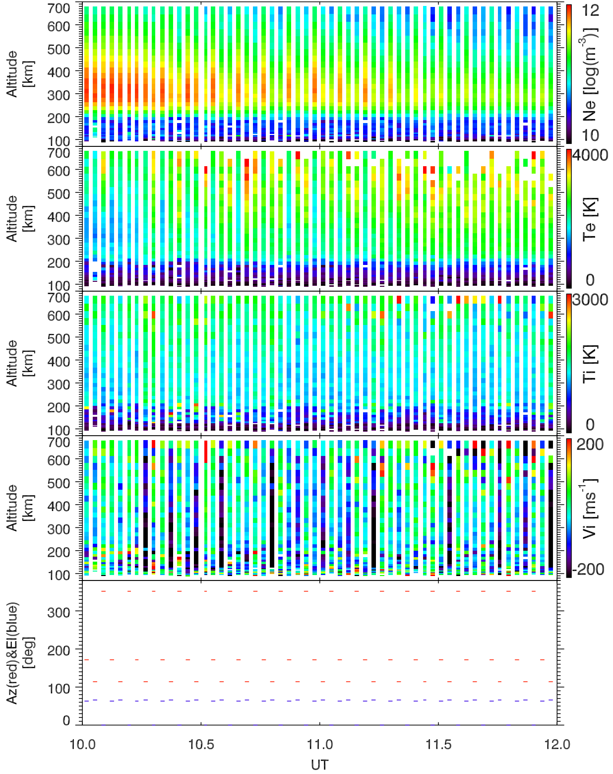
EISCAT 2002-10-20_10_12UT_tau0_ant@32m.
