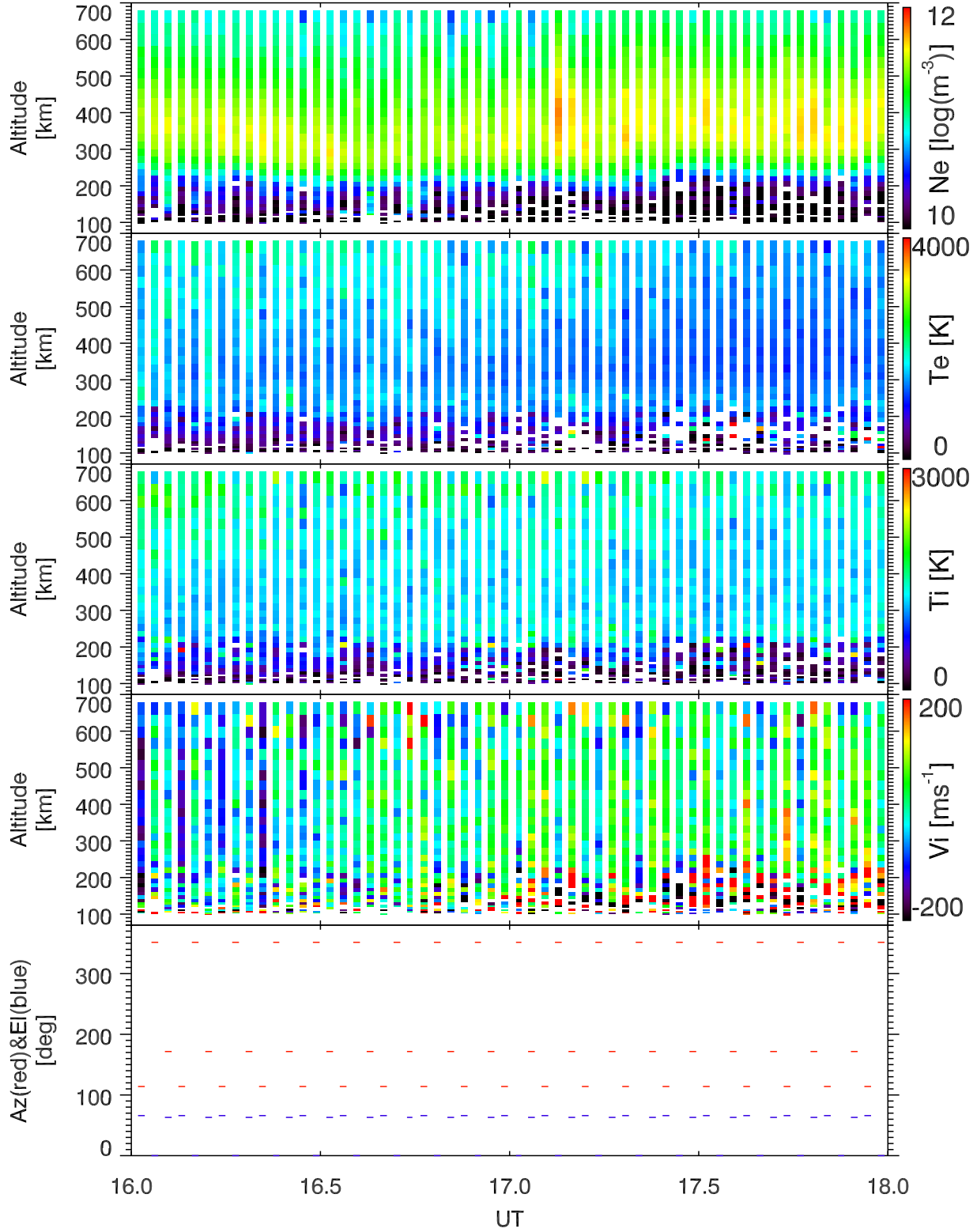
EISCAT 2002-10-21_16_18UT_tau0_ant@32m.
