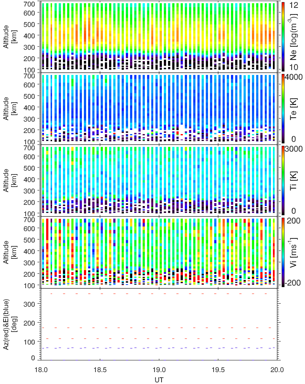
EISCAT 2002-10-21_18_20UT_tau0_ant@32m.
