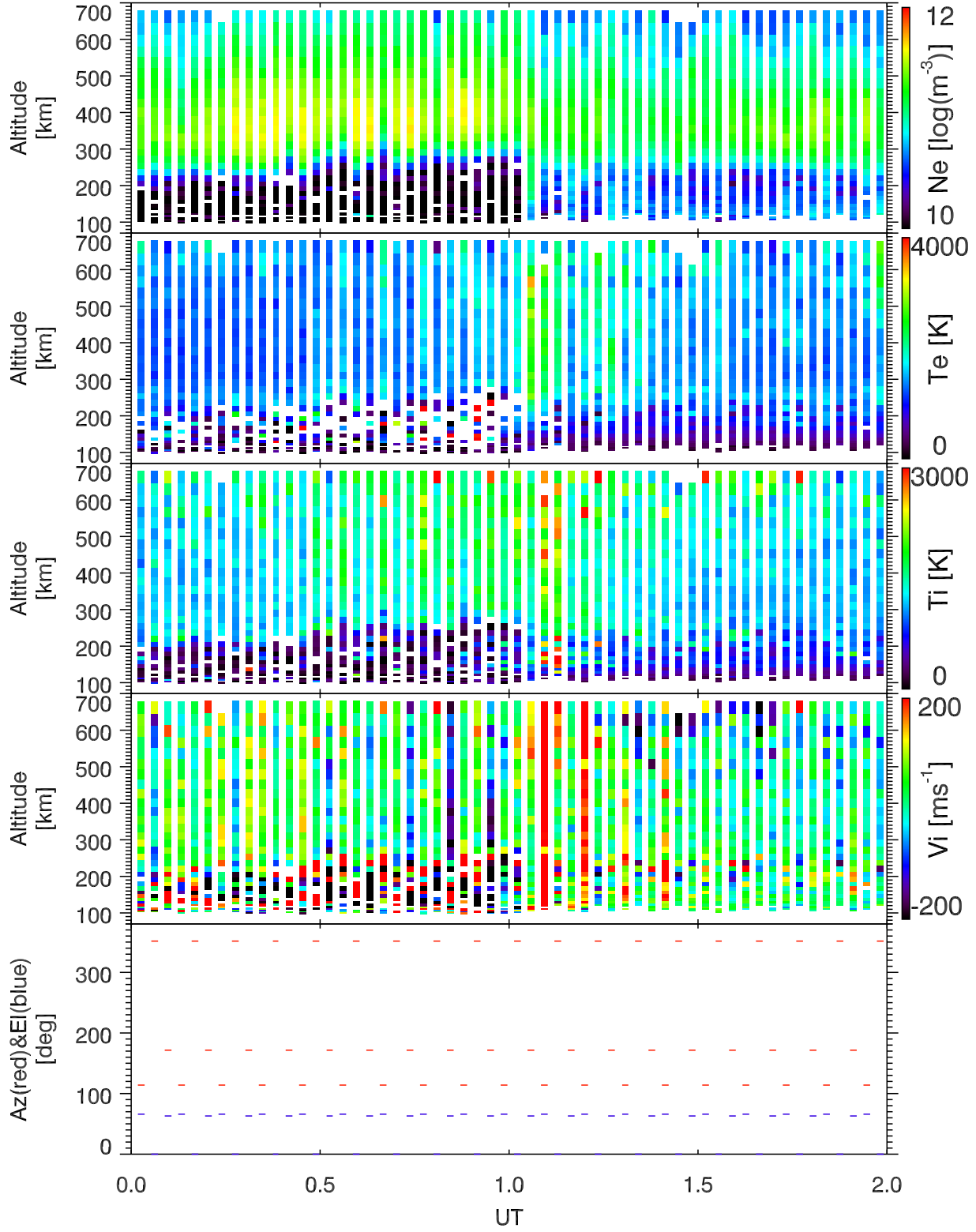
EISCAT 2002-10-22_00_02UT_tau0_ant@32m.
