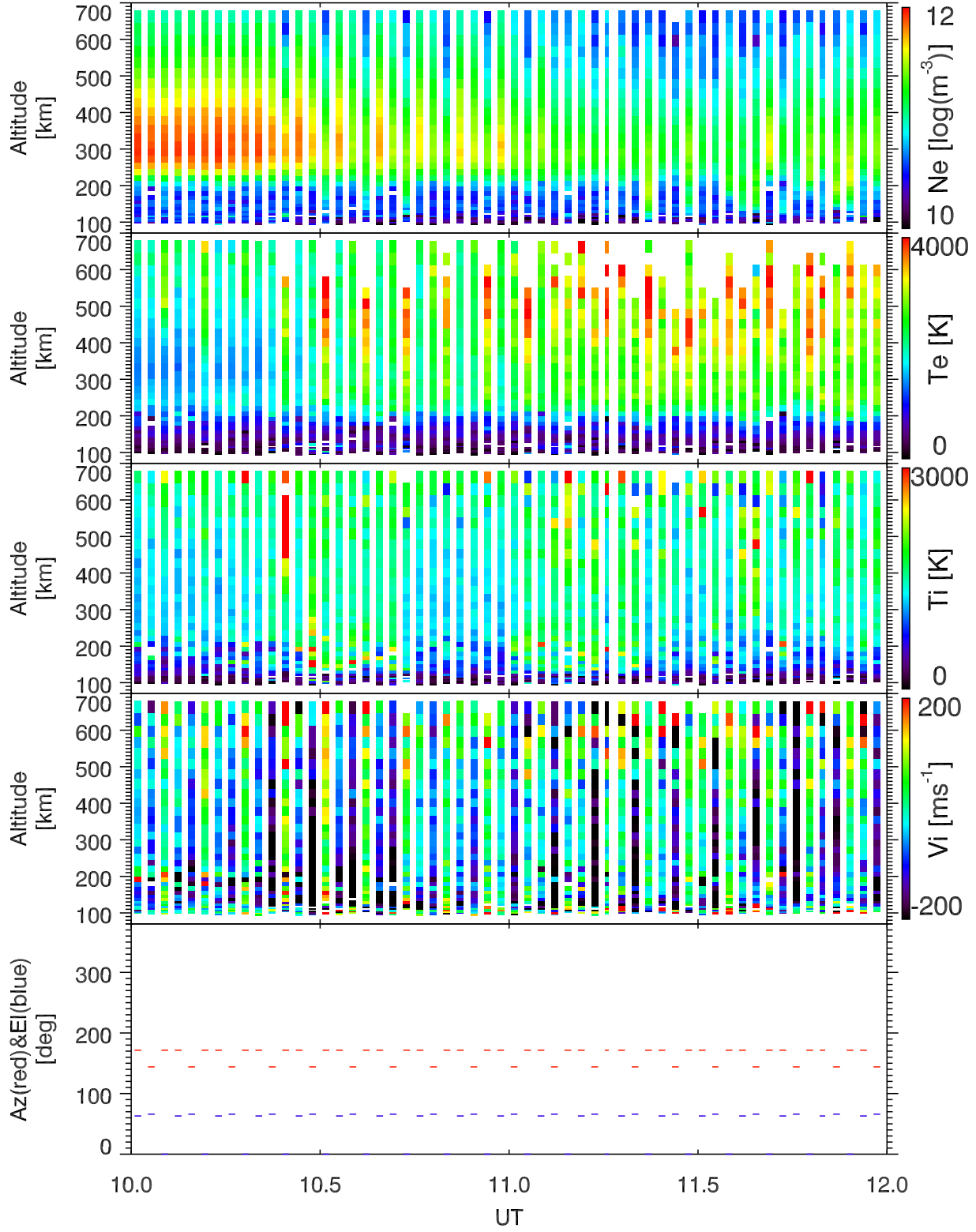
EISCAT 2002-10-23_10_12UT_tau0_ant@32m.
