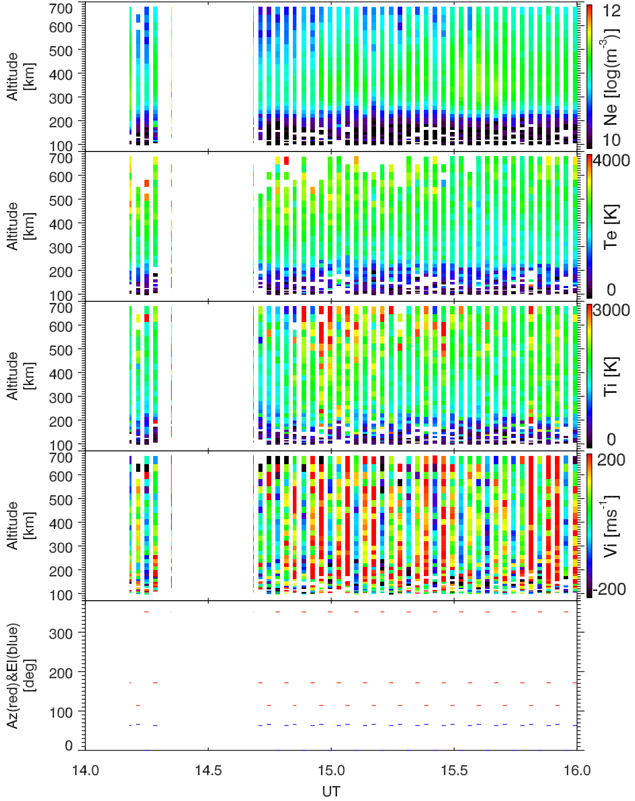
EISCAT 2002-10-24_14_16UT_tau0_ant@32m.
