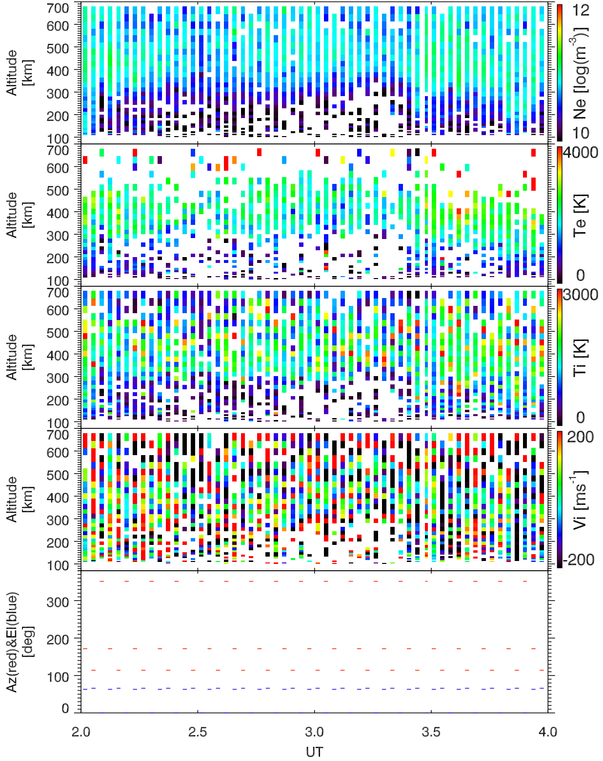
EISCAT 2002-10-25_02_04UT_tau0_ant@32m.
