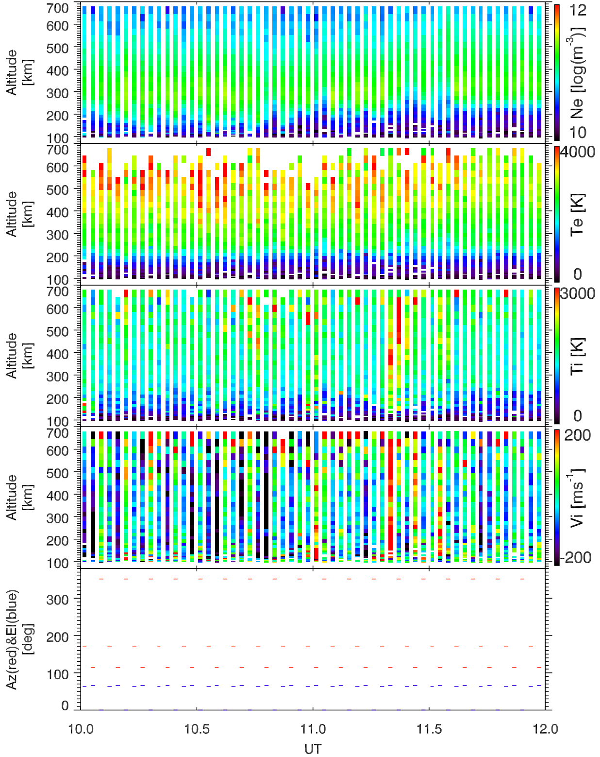
EISCAT 2002-10-25_10_12UT_tau0_ant@32m.
