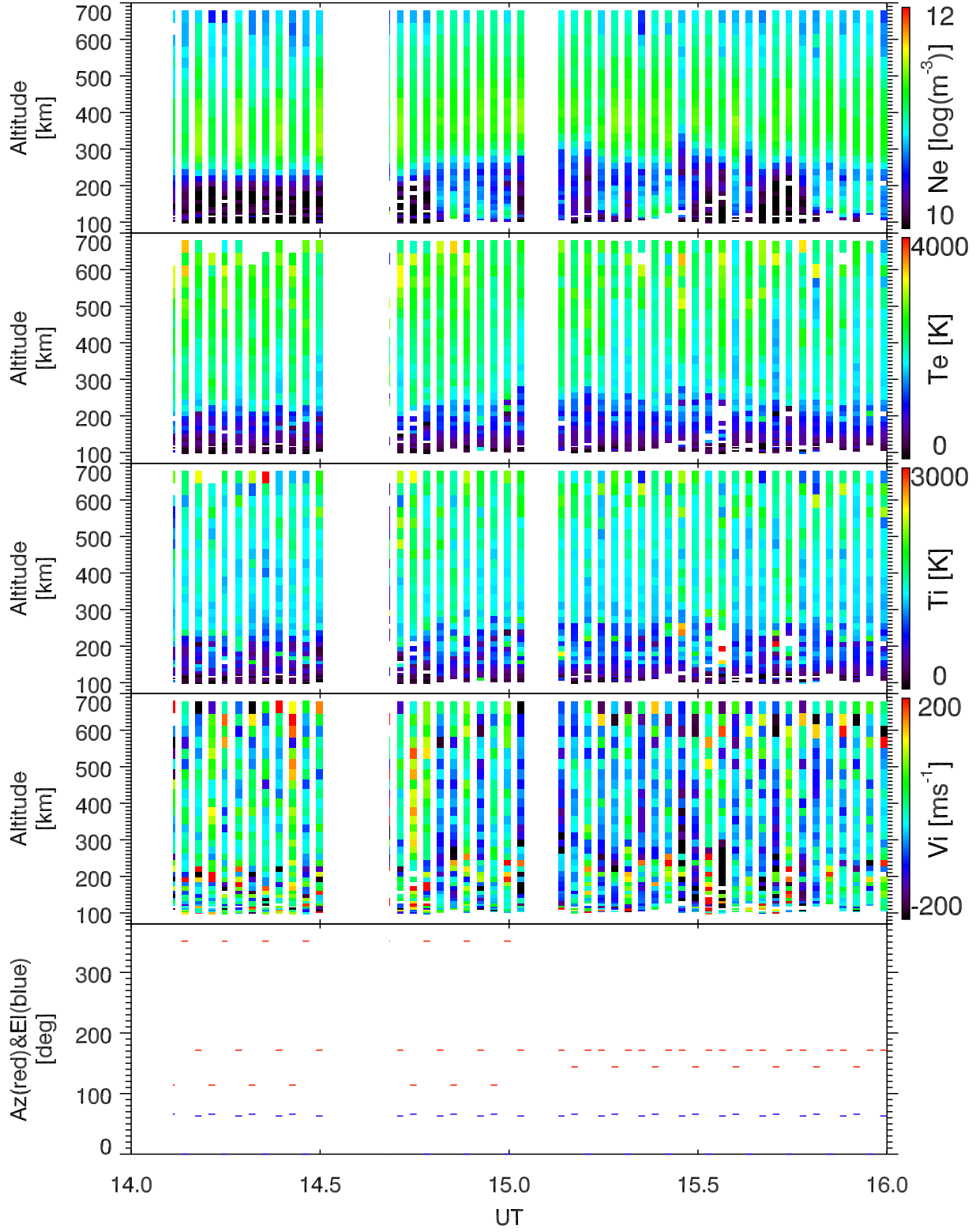
EISCAT 2002-10-25_14_16UT_tau0_ant@32m.
