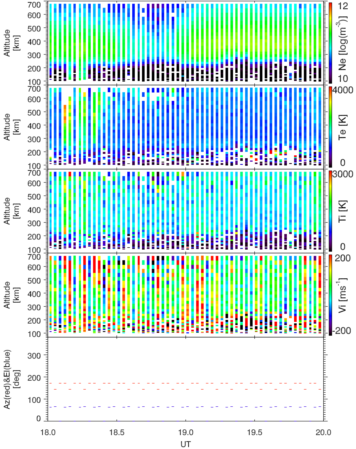
EISCAT 2002-10-25_18_20UT_tau0_ant@32m.
