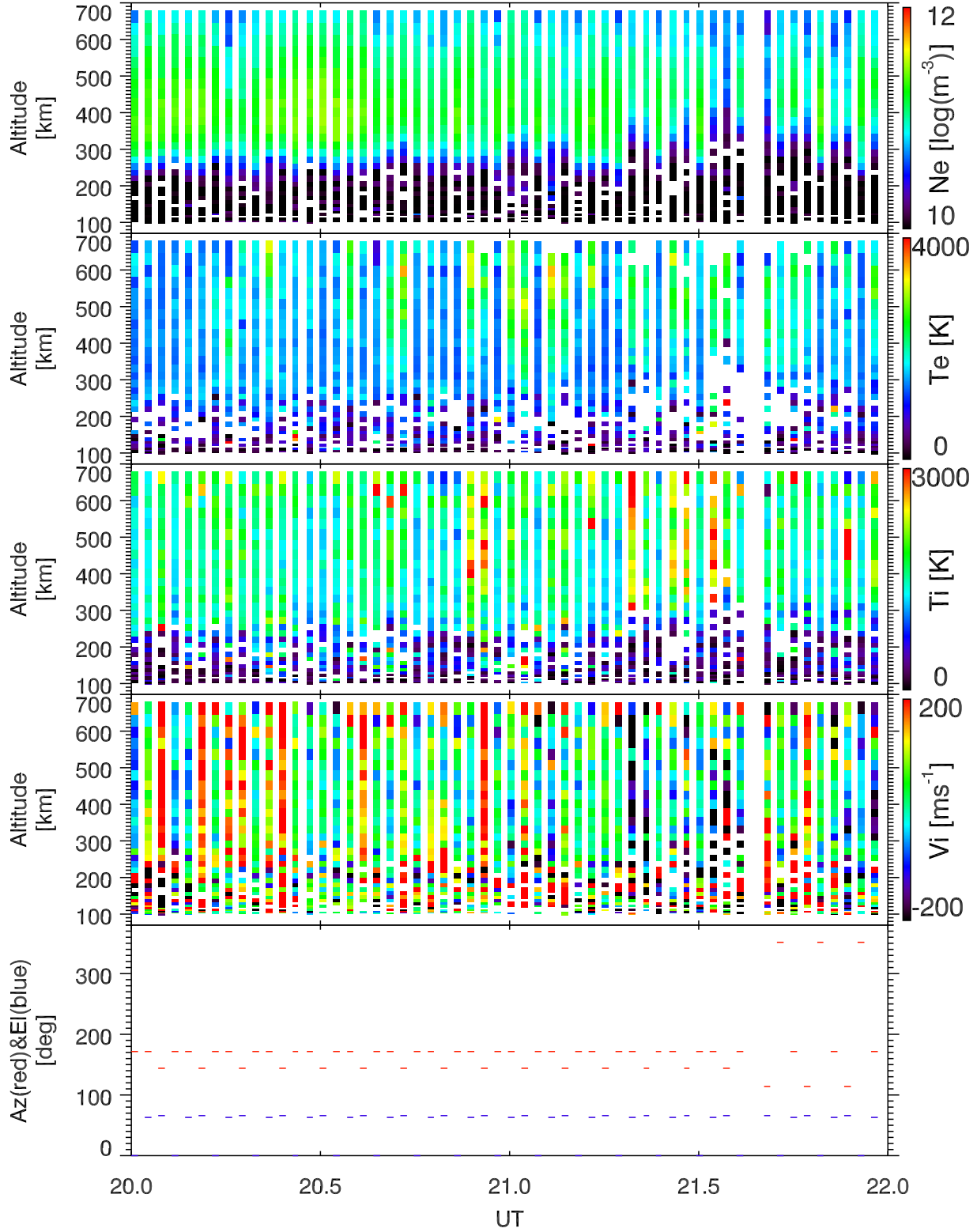
EISCAT 2002-10-25_20_22UT_tau0_ant@32m.
