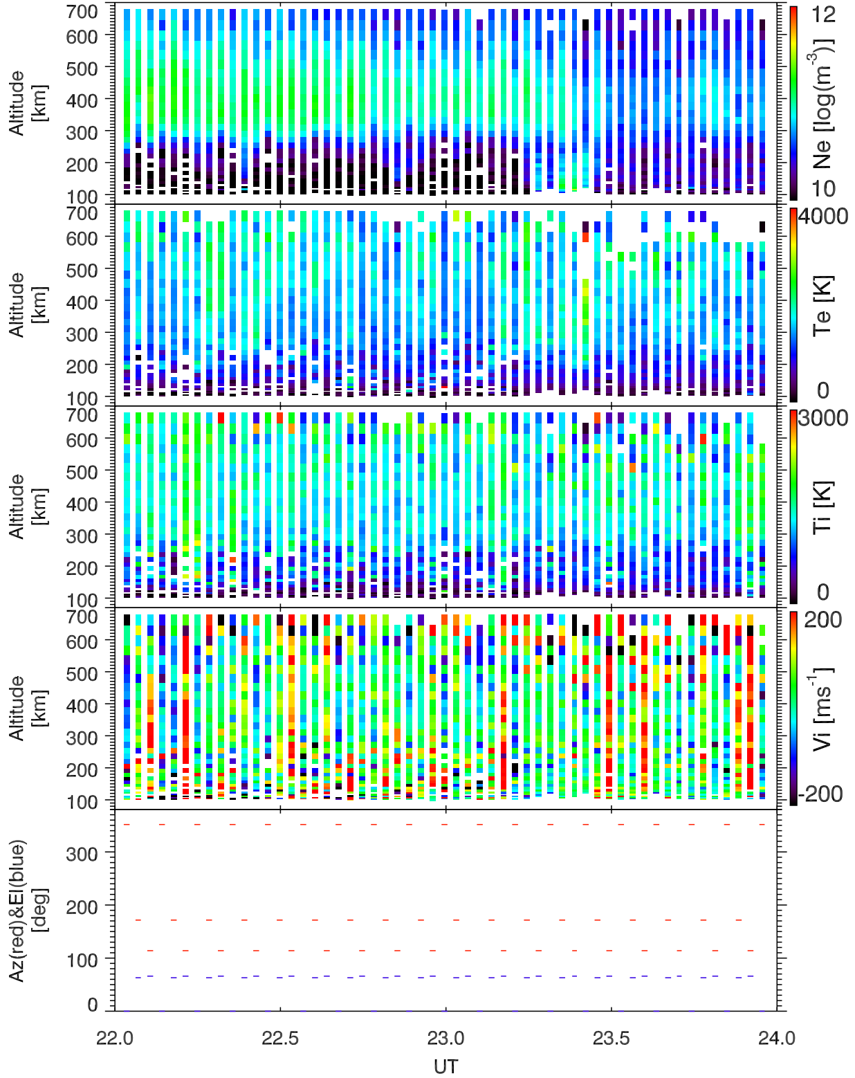
EISCAT 2002-10-25_22_24UT_tau0_ant@32m.
