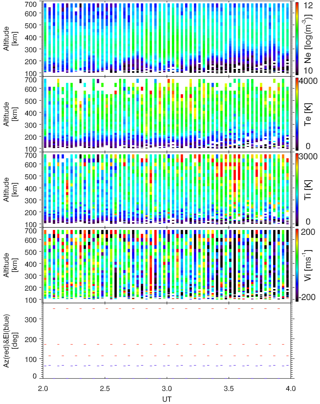
EISCAT 2002-10-26_02_04UT_tau0_ant@32m.
