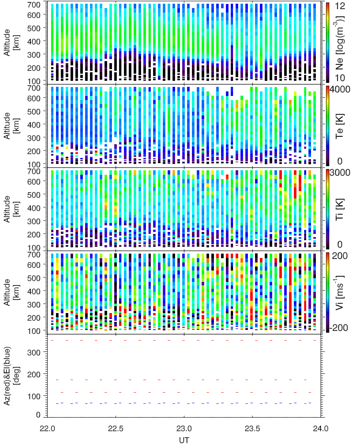
EISCAT 2002-10-26_22_24UT_tau0_ant@32m.
