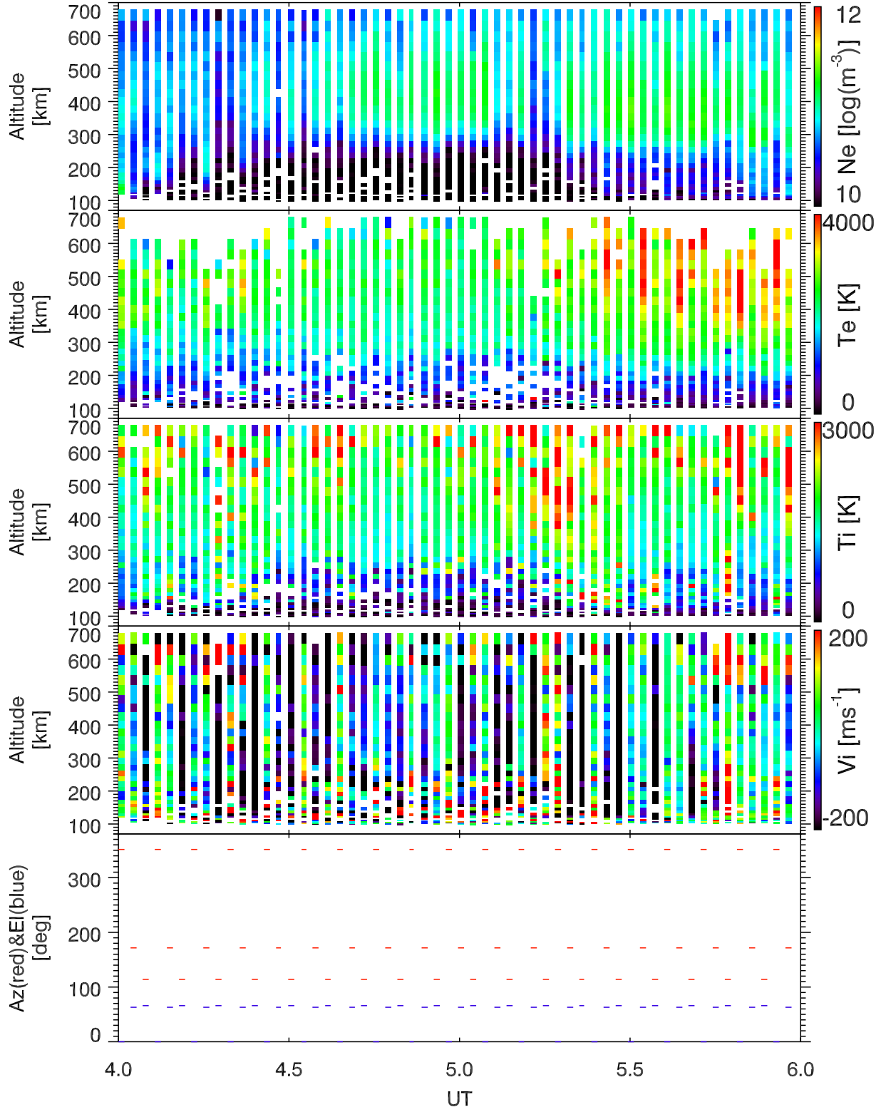
EISCAT 2002-10-27_04_06UT_tau0_ant@32m.
