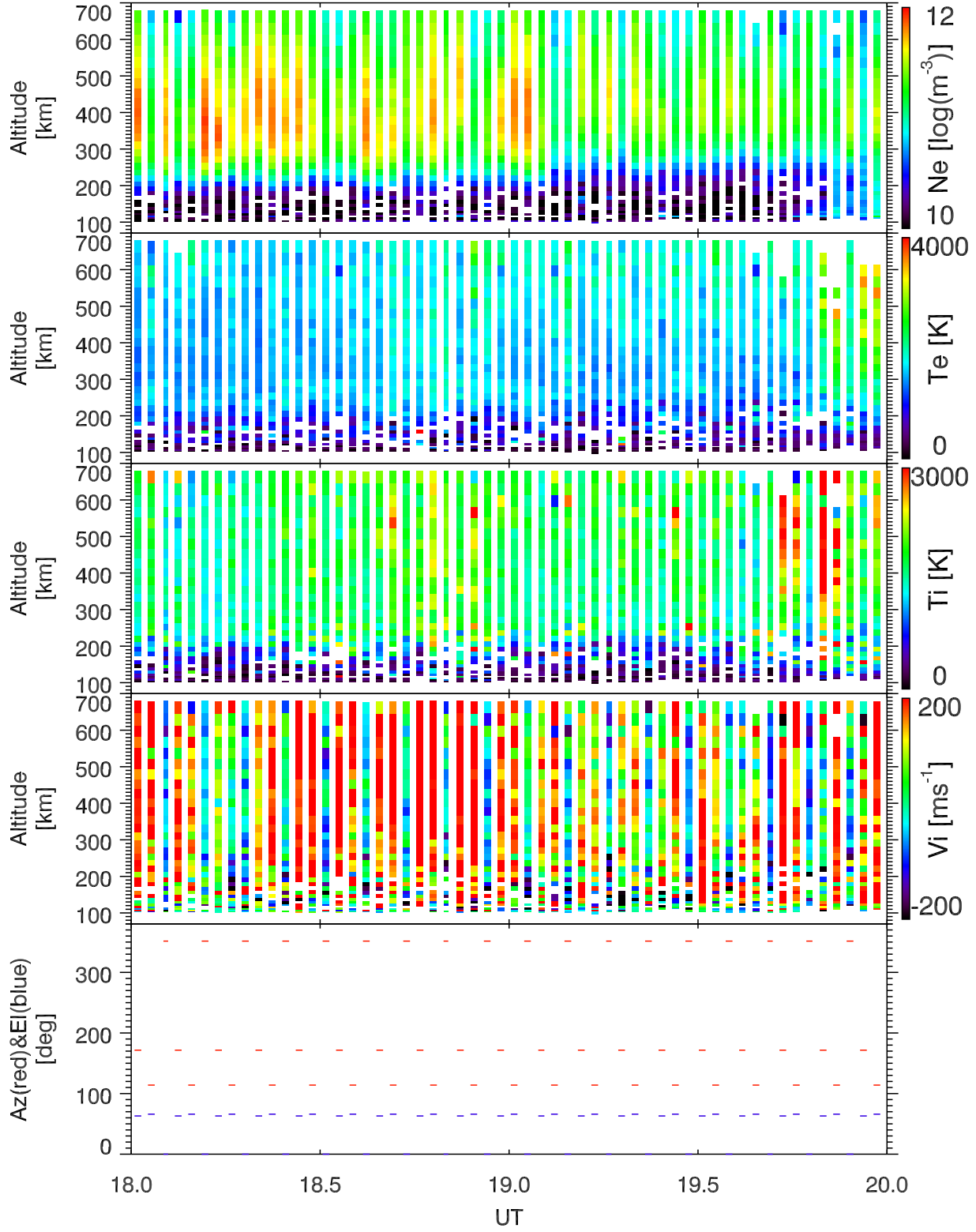
EISCAT 2002-10-27_18_20UT_tau0_ant@32m.
