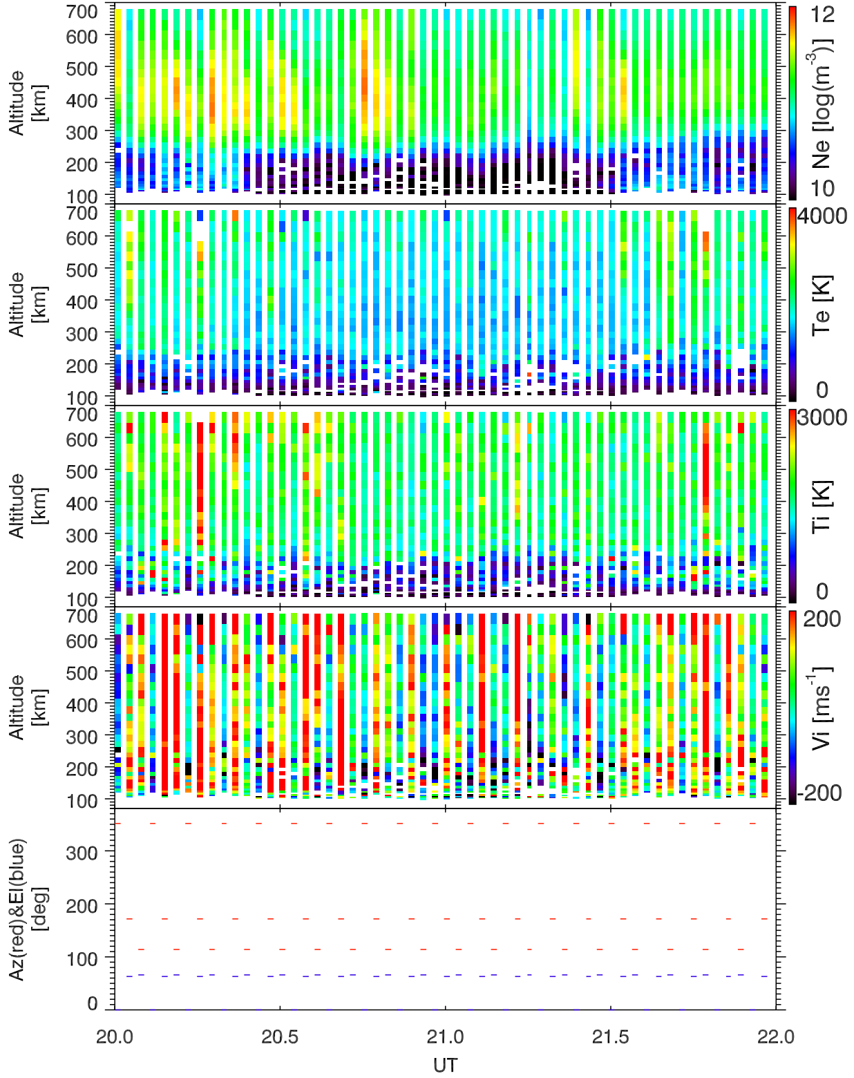
EISCAT 2002-10-27_20_22UT_tau0_ant@32m.
