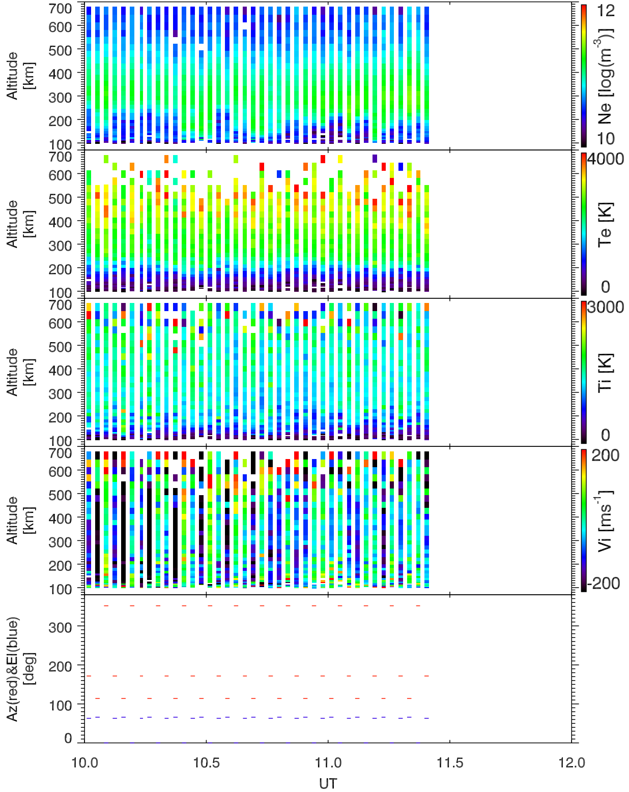
EISCAT 2002-10-28_10_12UT_tau0_ant@32m.
