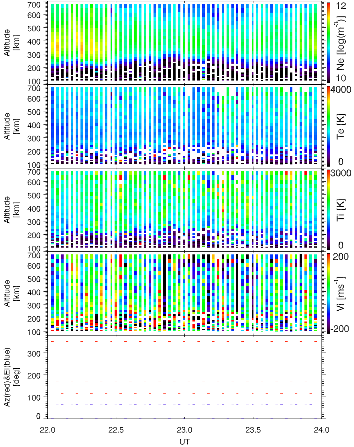
EISCAT 2002-10-28_22_24UT_tau0_ant@32m.
