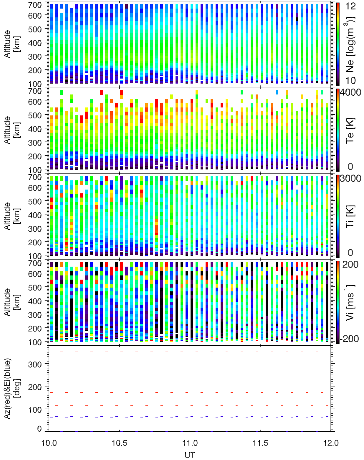
EISCAT 2002-10-29_10_12UT_tau0_ant@32m.
