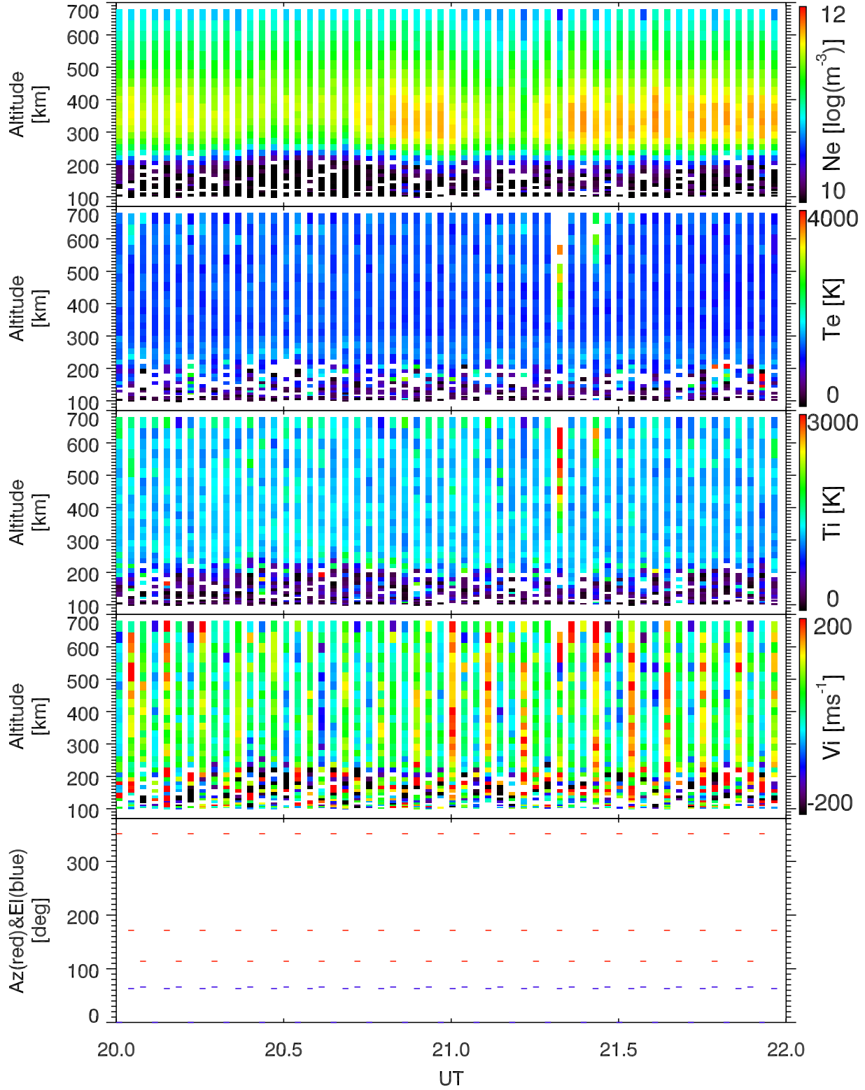
EISCAT 2002-10-29_20_22UT_tau0_ant@32m.
