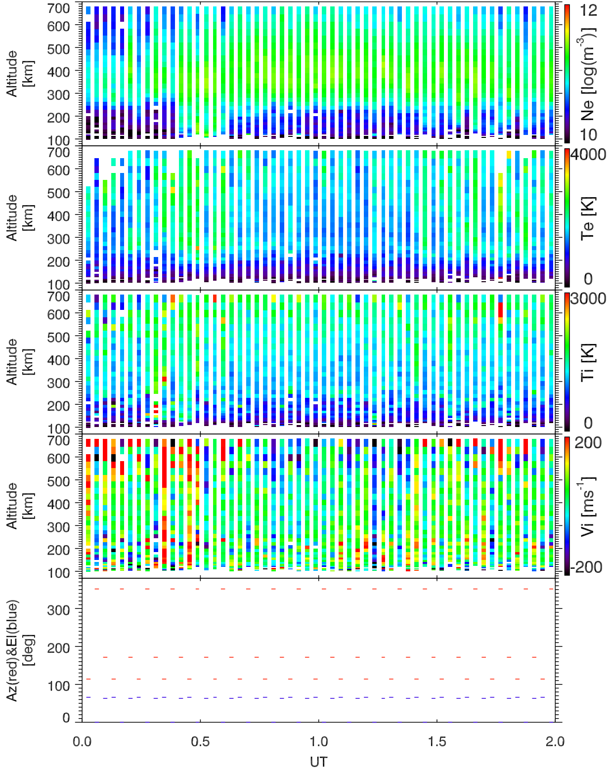
EISCAT 2002-10-30_00_02UT_tau0_ant@32m.
