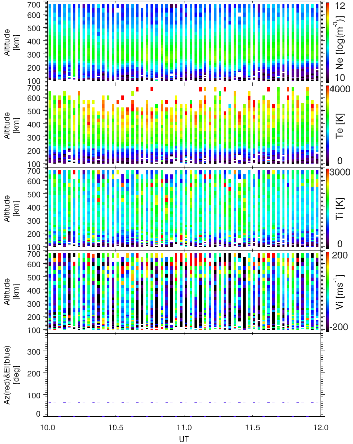
EISCAT 2002-10-31_10_12UT_tau0_ant@32m.
