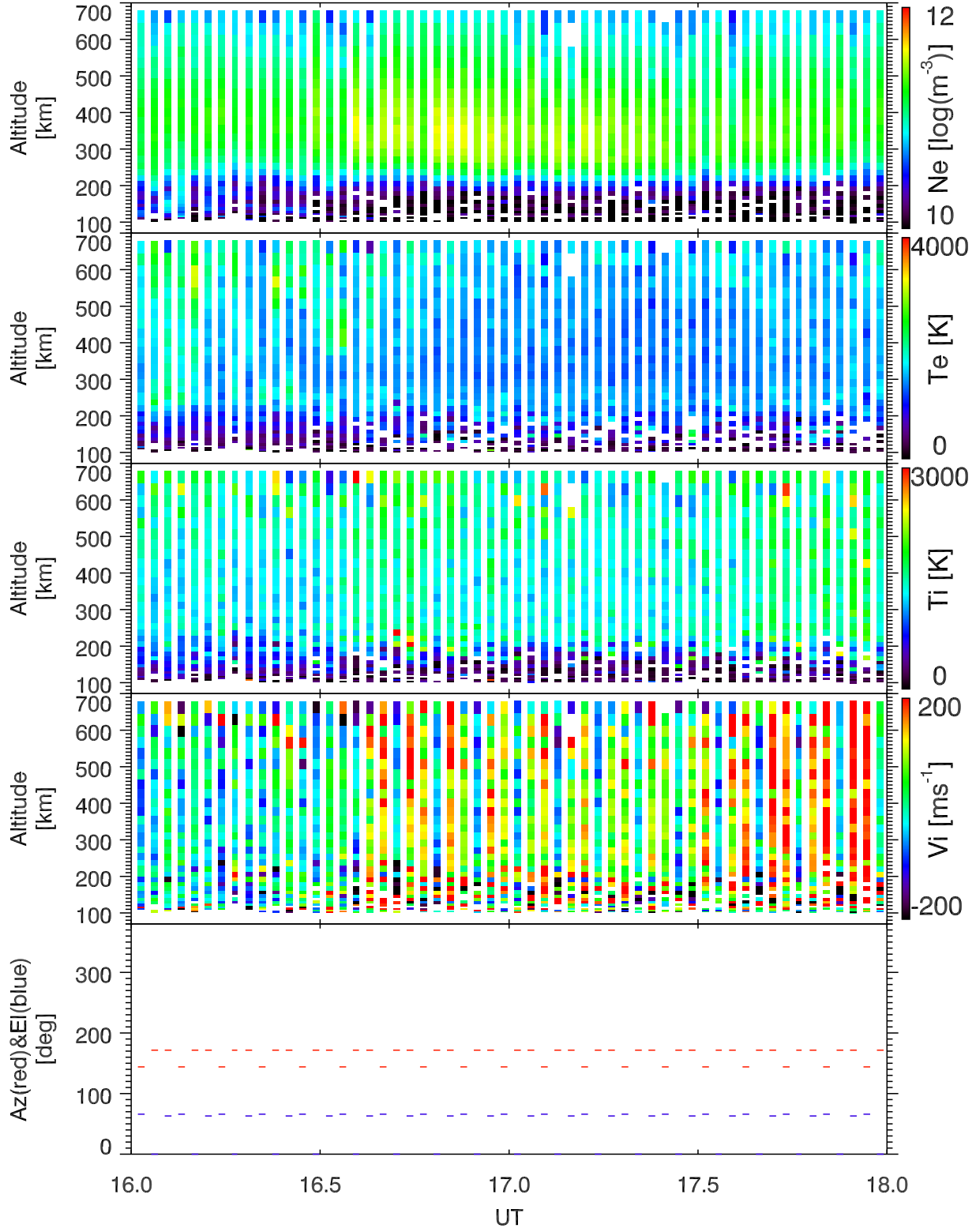
EISCAT 2002-10-31_16_18UT_tau0_ant@32m.
