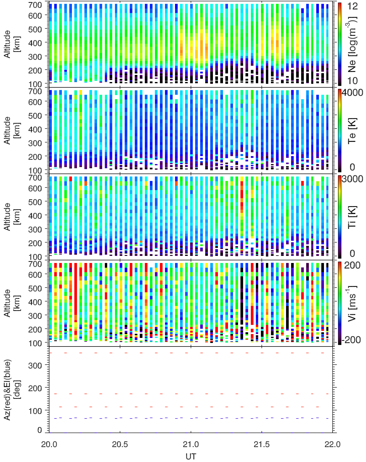
EISCAT 2002-11-01_20_22UT_tau0_ant@32m.
