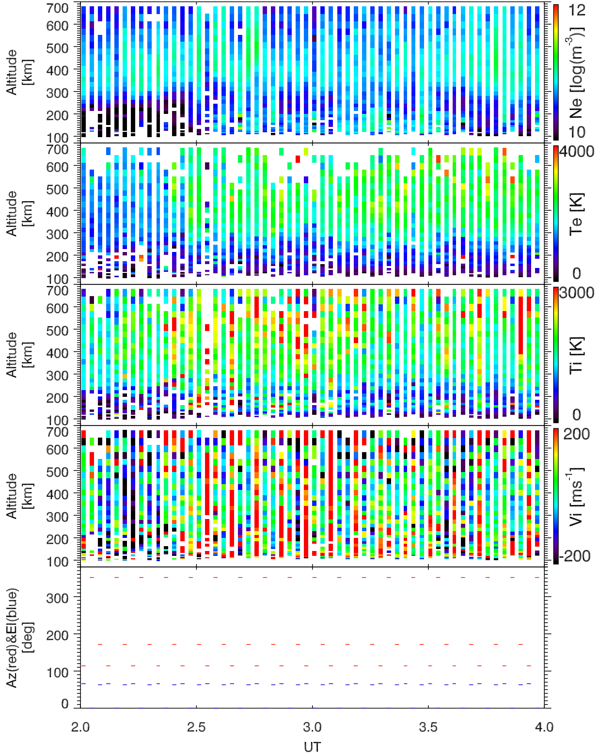
EISCAT 2002-11-13_02_04UT_tau0_ant@32m.
