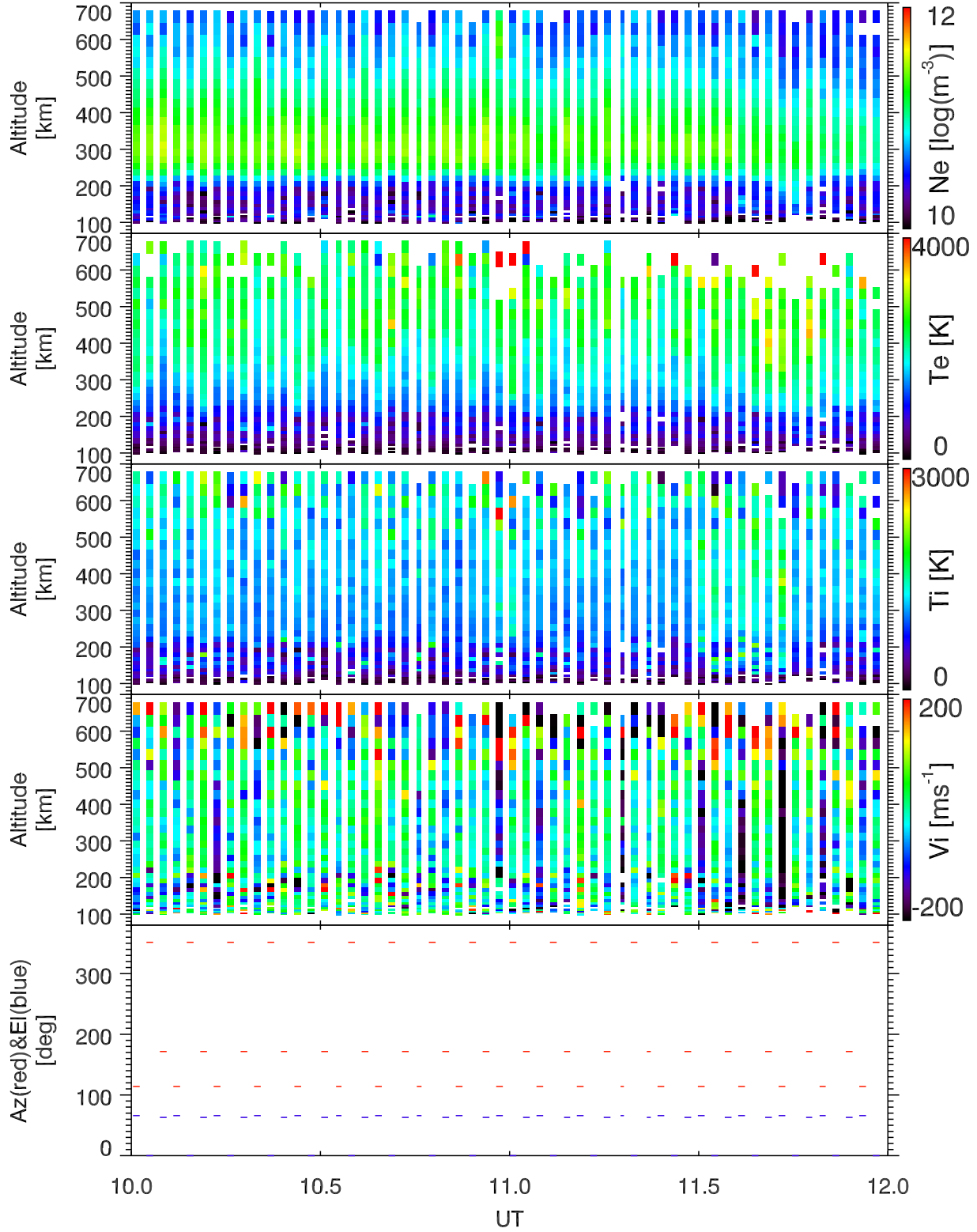
EISCAT 2002-11-14_10_12UT_tau0_ant@32m.
