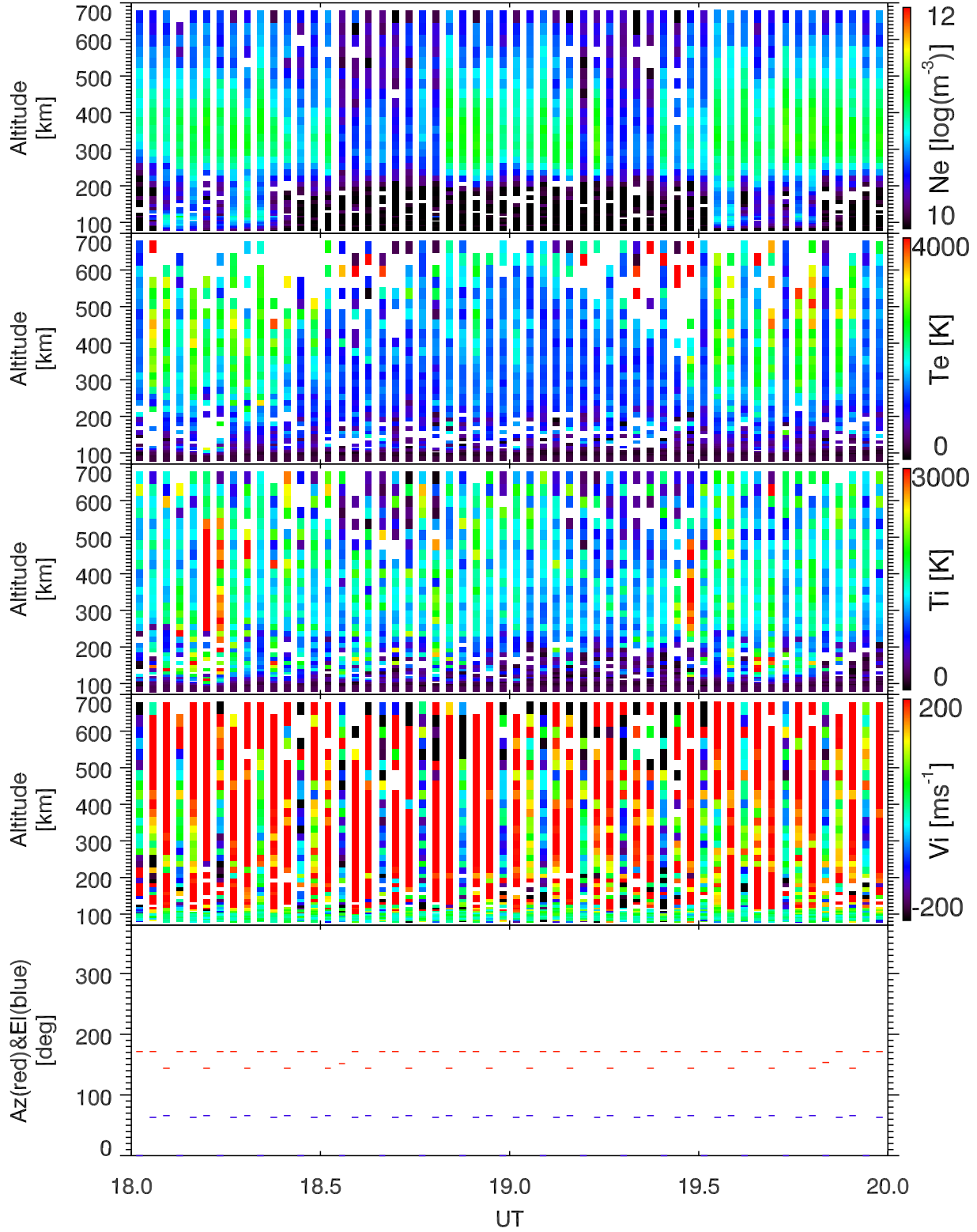
EISCAT 2003-11-12_18_20UT_steffe_ant@32m.
