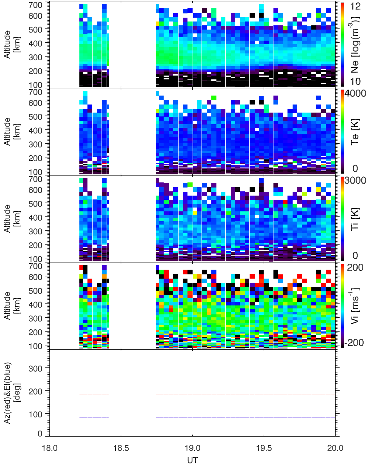
EISCAT 2004-02-19_18_20UT_steffe_120@42m.
