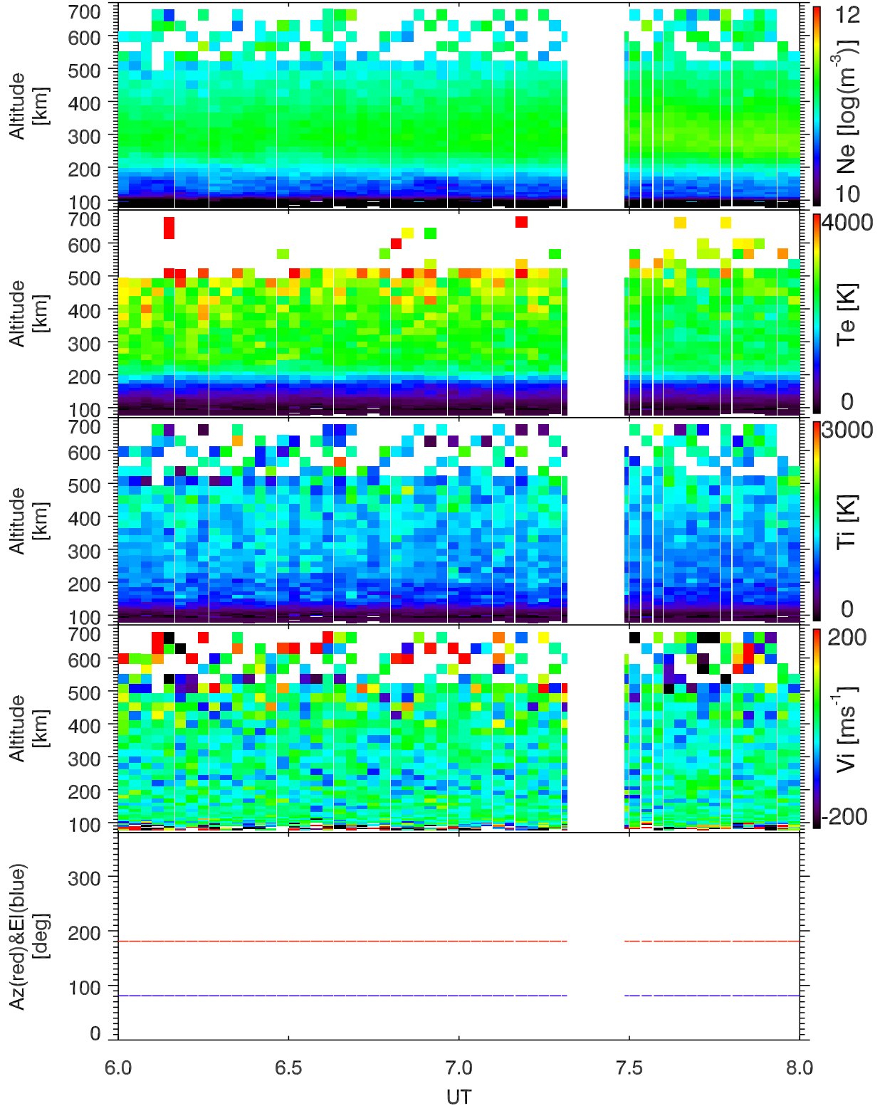
EISCAT 2004-03-25_06_08UT_steffe_120@42m.
