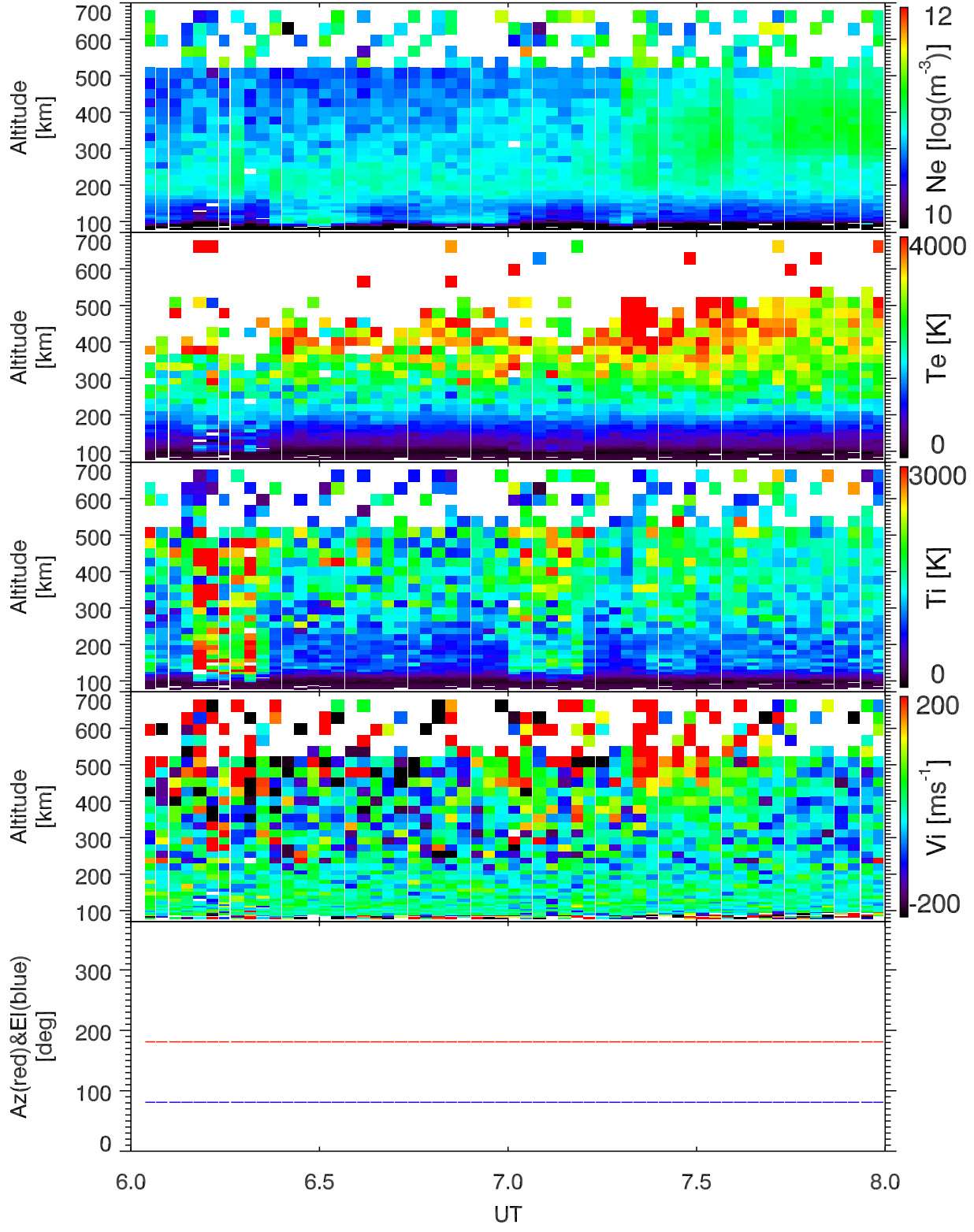
EISCAT 2004-04-25_06_08UT_steffe_120@42m.
