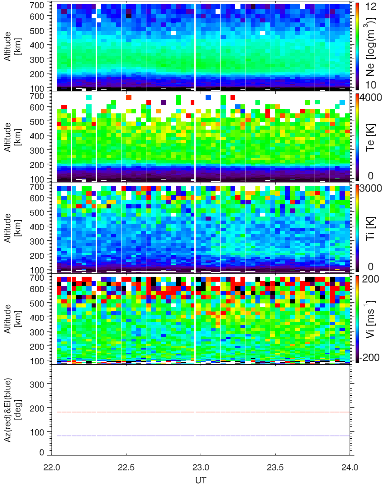
EISCAT 2004-05-24_22_24UT_steffe_120@42m.
