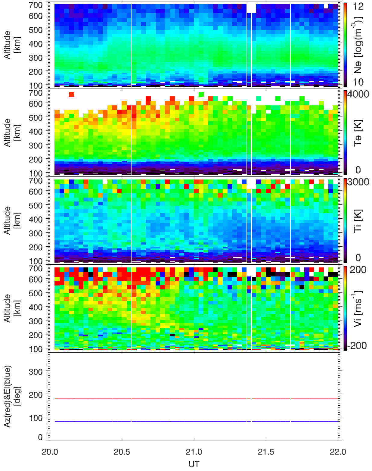
EISCAT 2004-06-01_20_22UT_tau0_120@42m.
