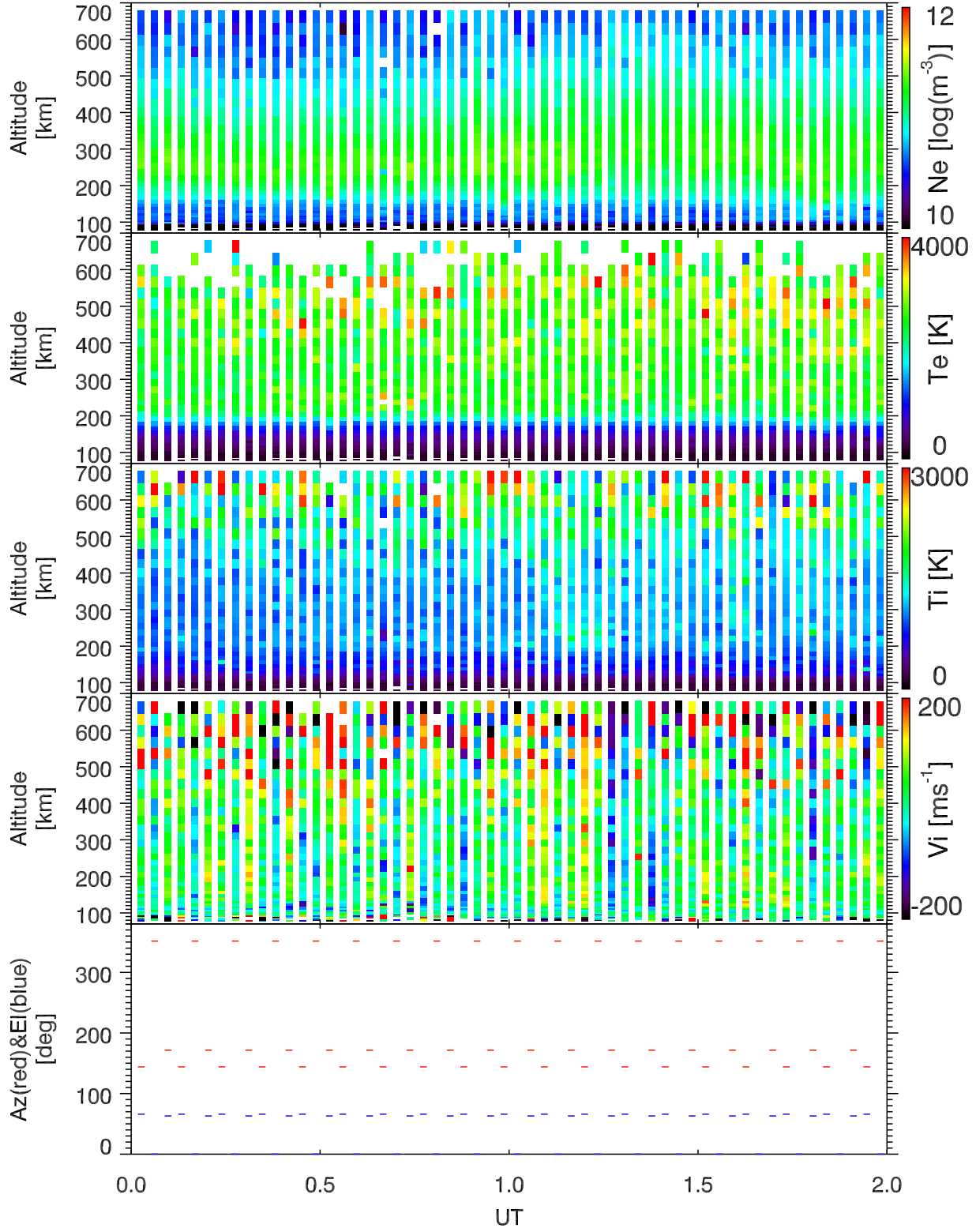
EISCAT 2004-06-05_00_02UT_steffe_ant@32m.
