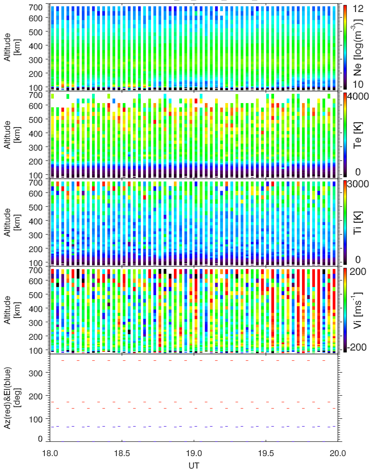
EISCAT 2004-06-07_18_20UT_steffe_ant@32m.
