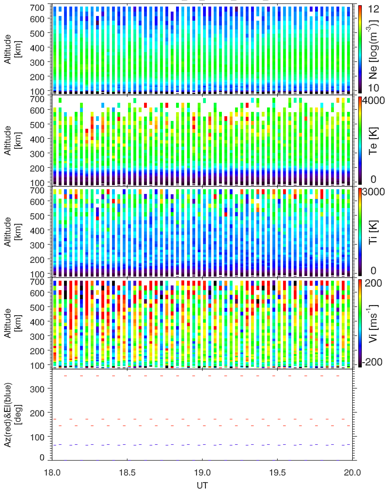
EISCAT 2004-06-09_18_20UT_steffe_ant@32m.
