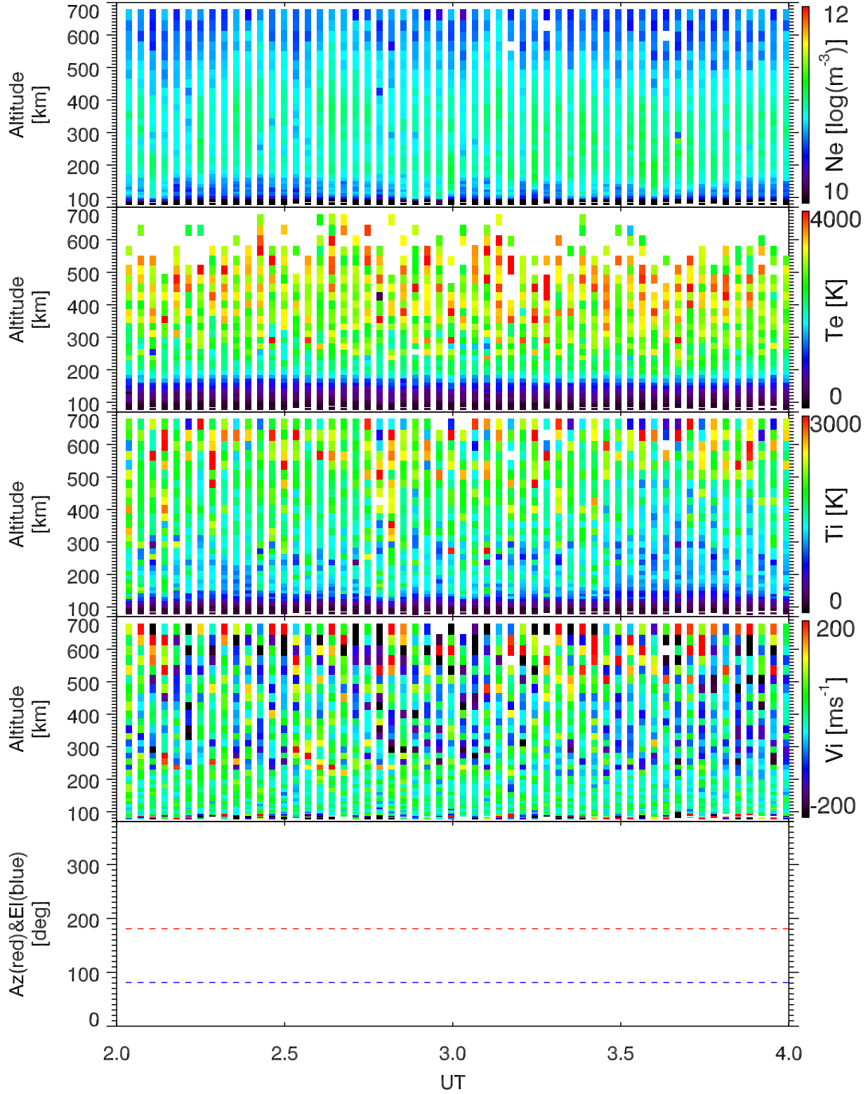
EISCAT 2004-06-10_02_04UT_steffe_ant@42m.
