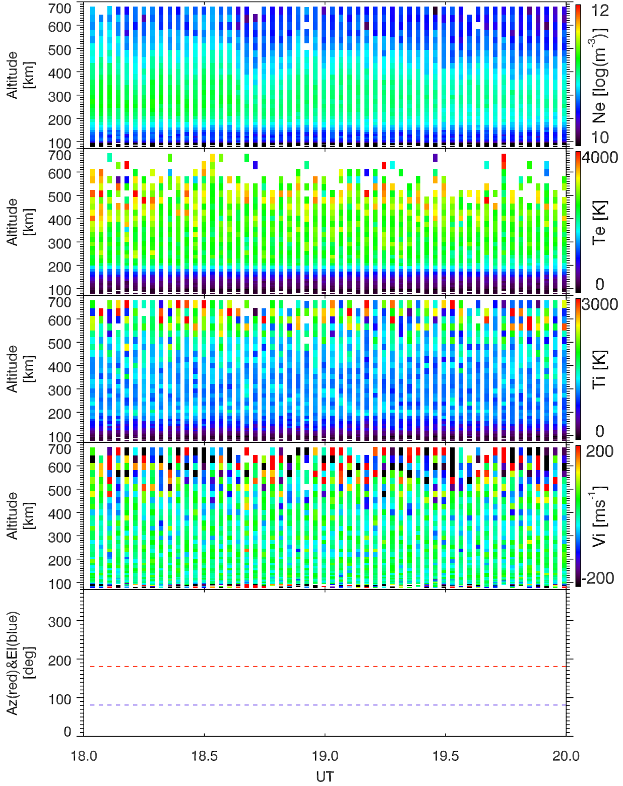
EISCAT 2004-06-10_18_20UT_steffe_ant@42m.
