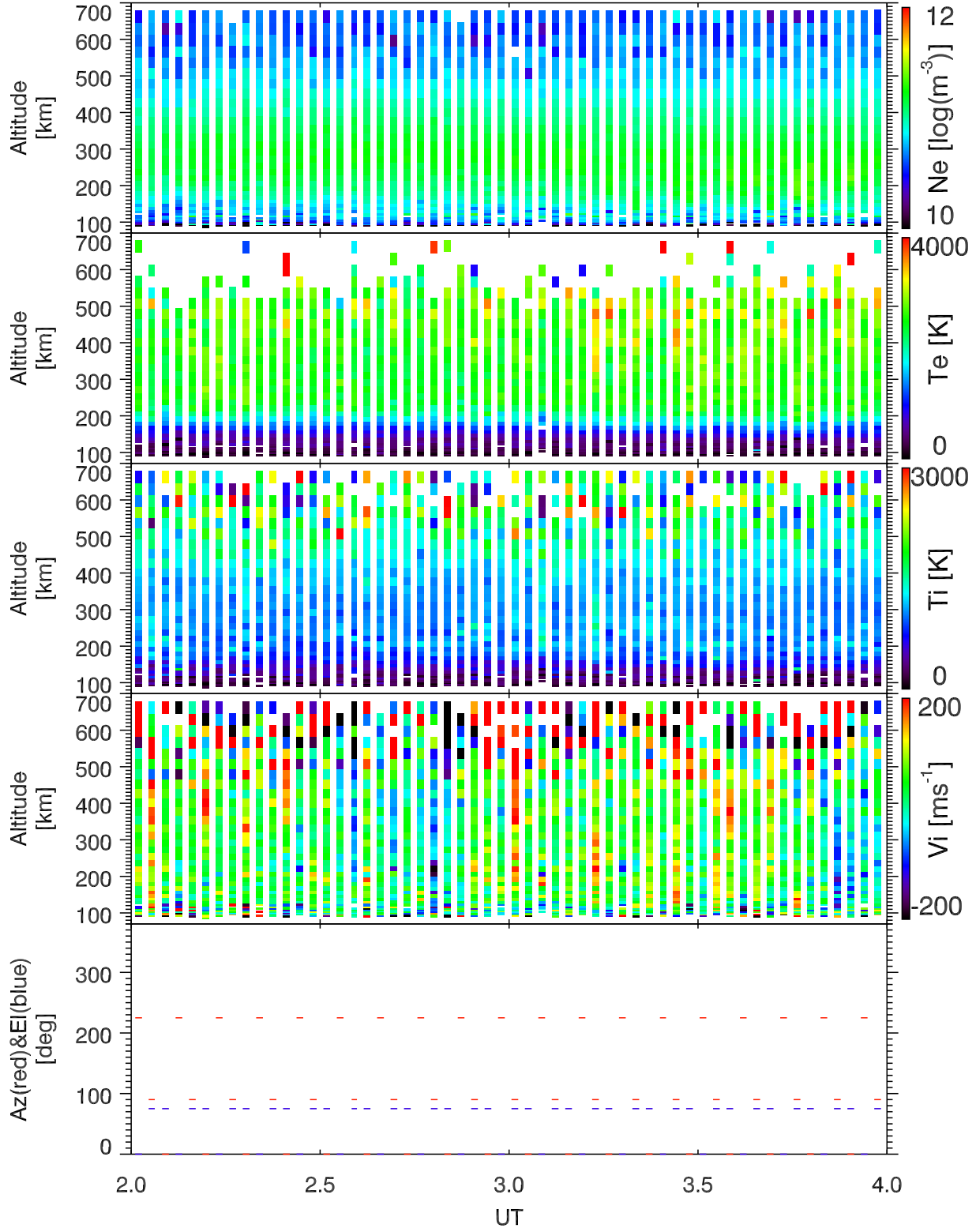
EISCAT 2005-07-23_02_04UT_tau0_ant@32m.
