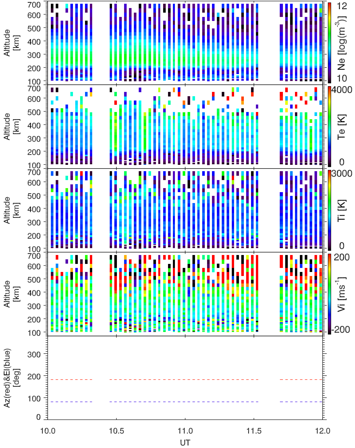
EISCAT 2005-11-09_10_12UT_tau0_ant@42m.
