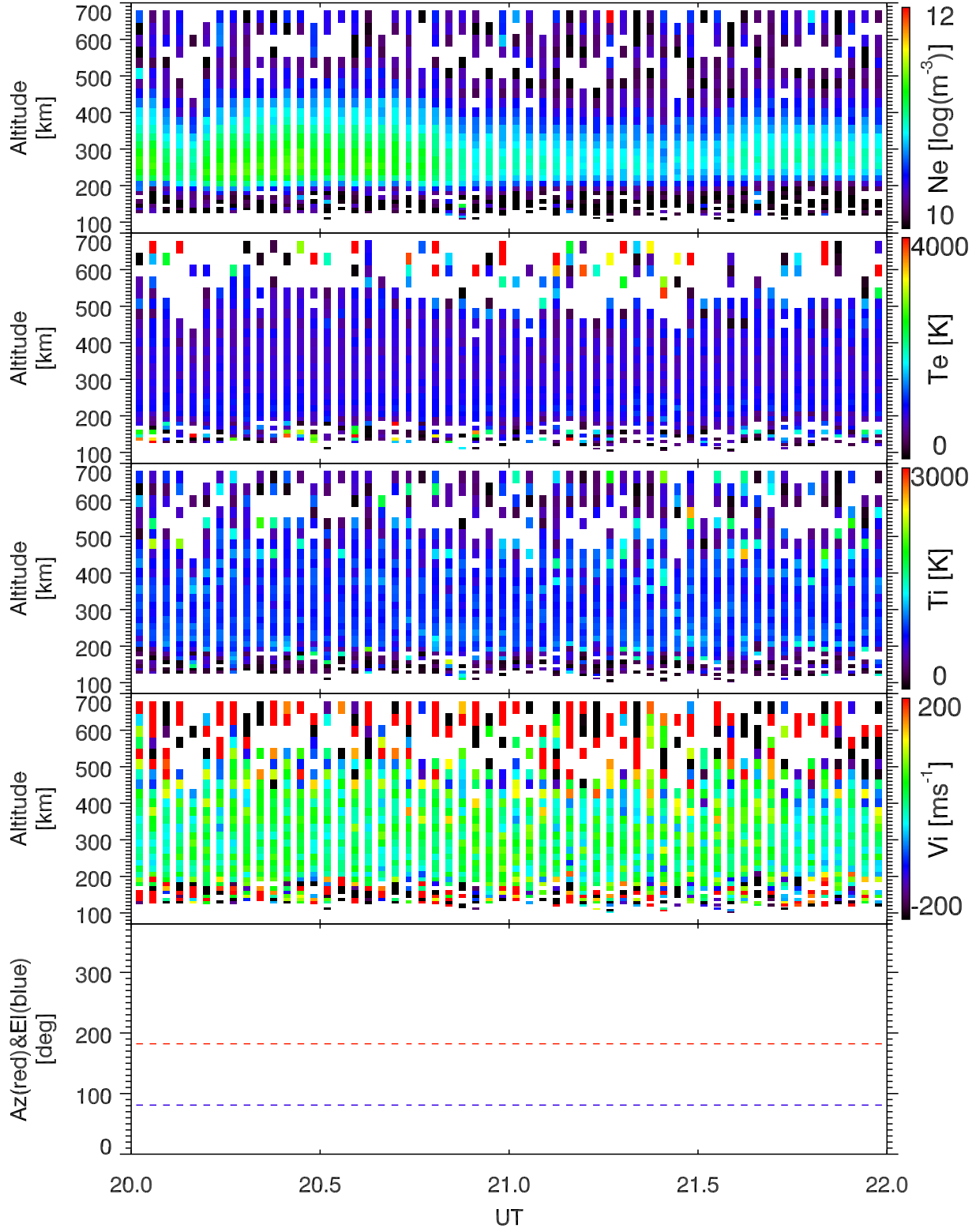
EISCAT 2005-11-10_20_22UT_tau0_ant@42m.
