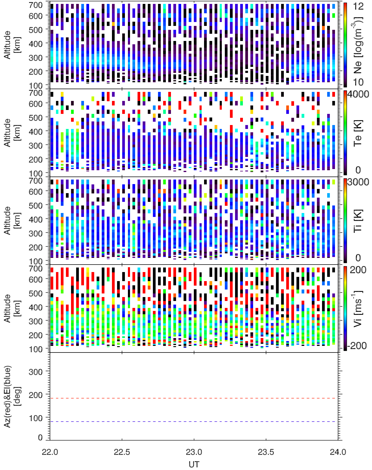
EISCAT 2005-11-10_22_24UT_tau0_ant@42m.
