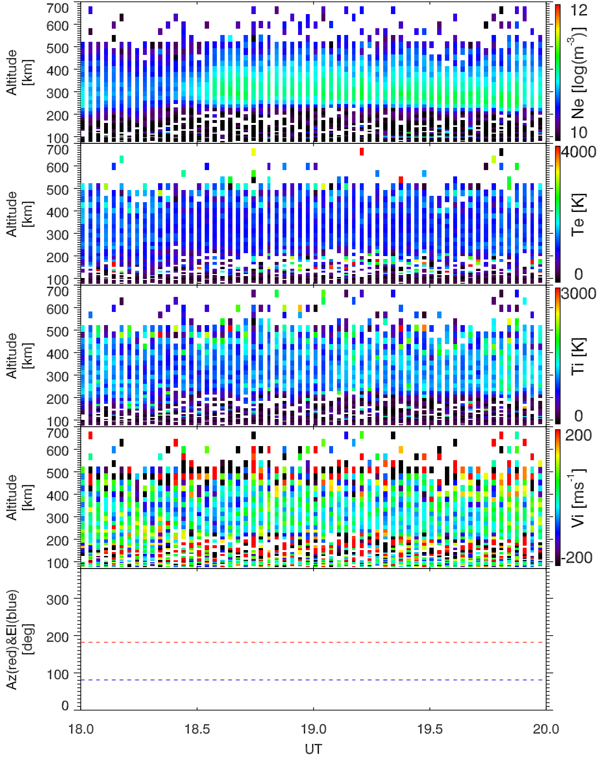
EISCAT 2006-02-20_18_20UT_steffe_120@42m.
