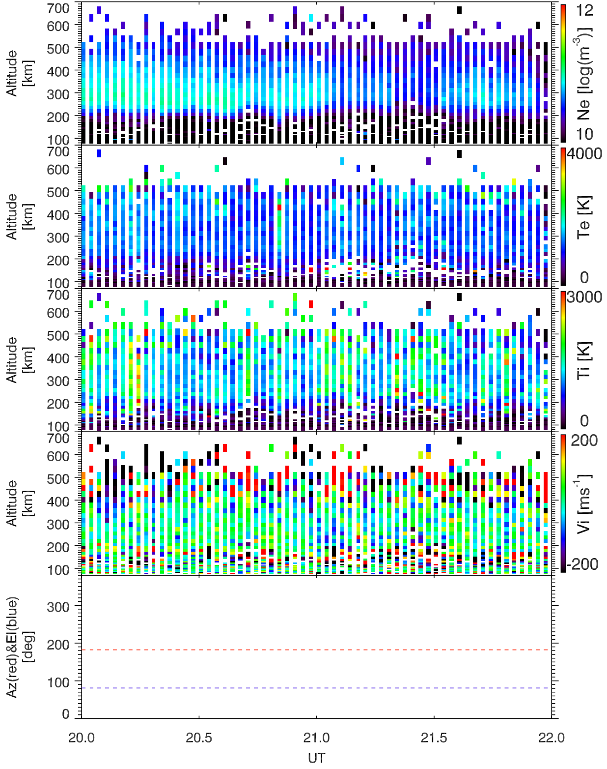
EISCAT 2006-02-21_20_22UT_steffe_120@42m.
