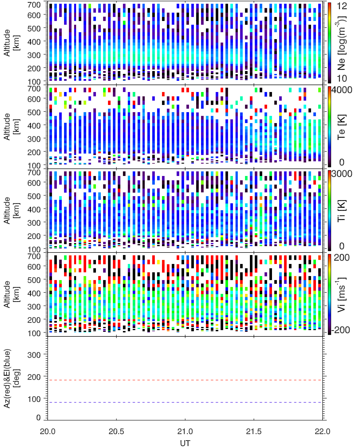
EISCAT 2006-09-21_20_22UT_tau0_ant@42m.
