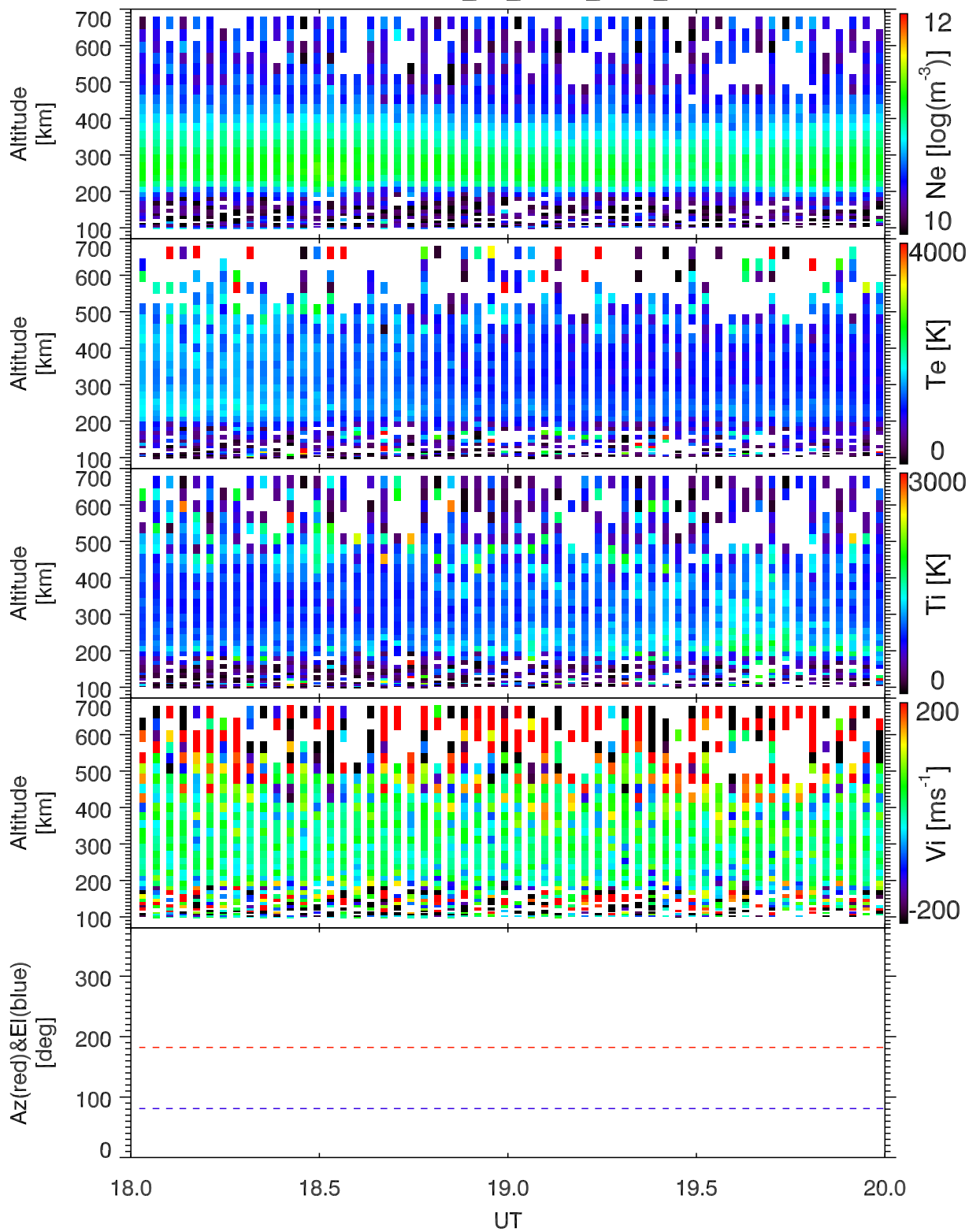
EISCAT 2006-09-22_18_20UT_tau0_ant@42m.
