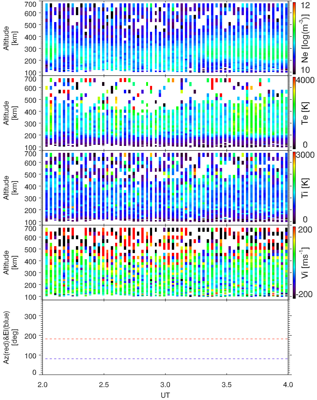
EISCAT 2006-09-23_02_04UT_tau0_ant@42m.
